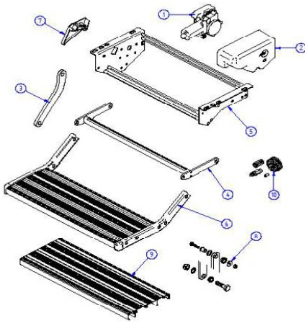
THULE Single step 12V ALU
